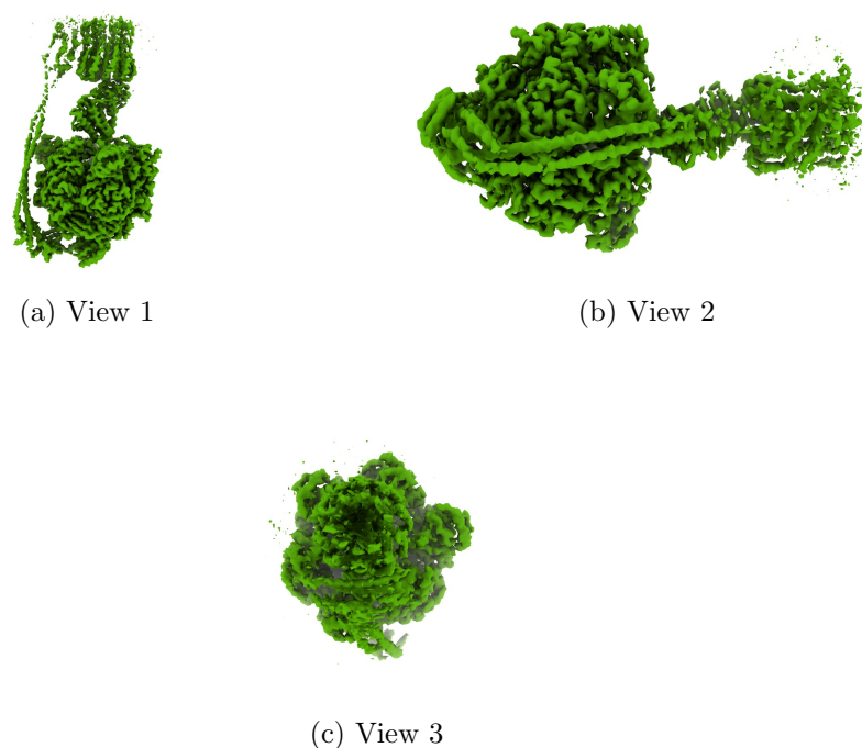
Figure 4: Isosurface at threshold=0.006230. Views generated by ChimeraX at a the following X, Y, Z angles: View 1 (0, -90, -90), View 2 (-90, 0, -90), View 3 (0, 0, 0).
