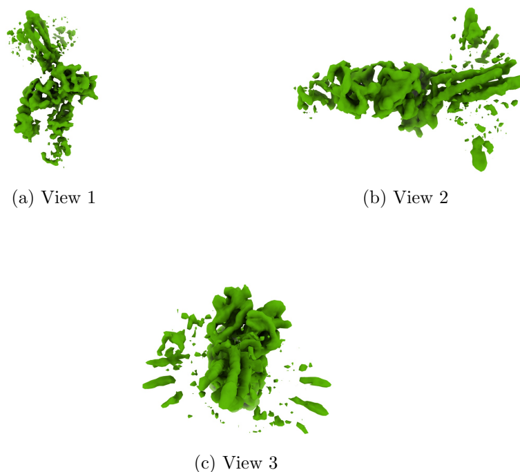
Figure 4: Isosurface at threshold=0.582000. Views generated by ChimeraX at a the following X, Y, Z angles: View 1 (0, -90, -90), View 2 (-90, 0, -90), View 3 (0, 0, 0).
