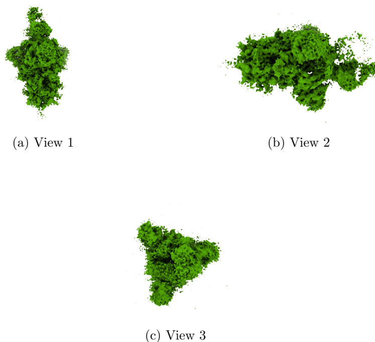
Figure 4: Isosurface at threshold=0.031900. Views generated by ChimeraX at a the following X, Y, Z angles: View 1 (0, -90, -90), View 2 (-90, 0, -90), View 3 (0, 0, 0).
