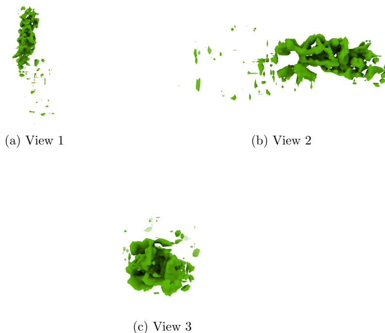
Figure 4: Isosurface at threshold=0.068600. Views generated by ChimeraX at a the following X, Y, Z angles: View 1 (0, -90, -90), View 2 (-90, 0, -90), View 3 (0, 0, 0).
