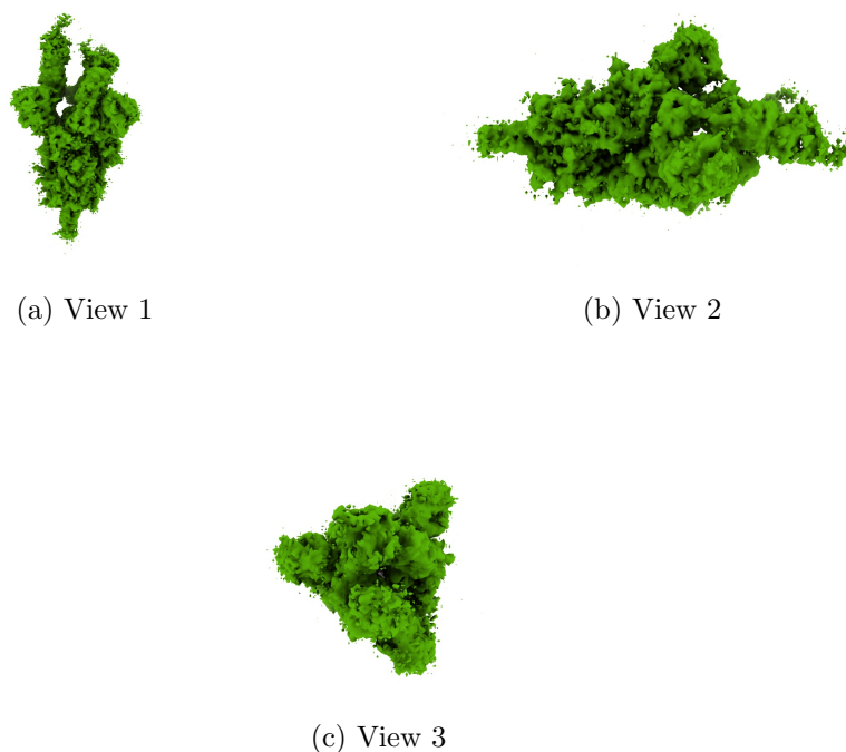
Figure 4: Isosurface at threshold=0.033400. Views generated by ChimeraX at a the following X, Y, Z angles: View 1 (0, -90, -90), View 2 (-90, 0, -90), View 3 (0, 0, 0).
