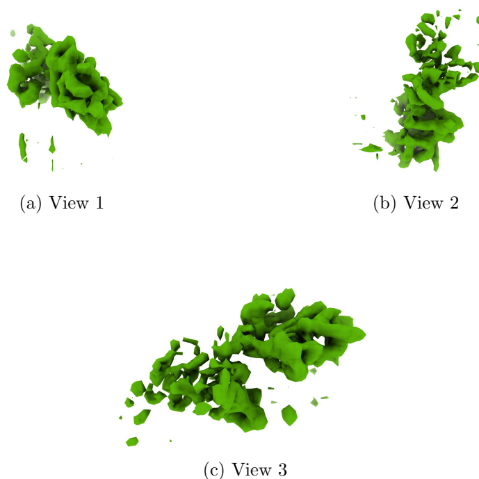
Figure 4: Isosurface at threshold=0.056300. Views generated by ChimeraX at a the following X, Y, Z angles: View 1 (0, -90, -90), View 2 (-90, 0, -90), View 3 (0, 0, 0).
