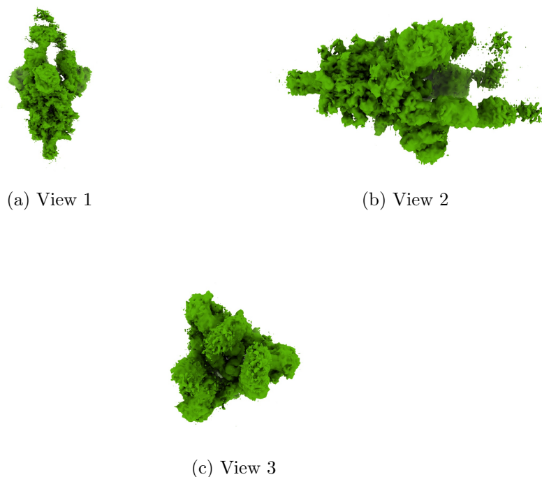
Figure 4: Isosurface at threshold=0.022400. Views generated by ChimeraX at a the following X, Y, Z angles: View 1 (0, -90, -90), View 2 (-90, 0, -90), View 3 (0, 0, 0).
