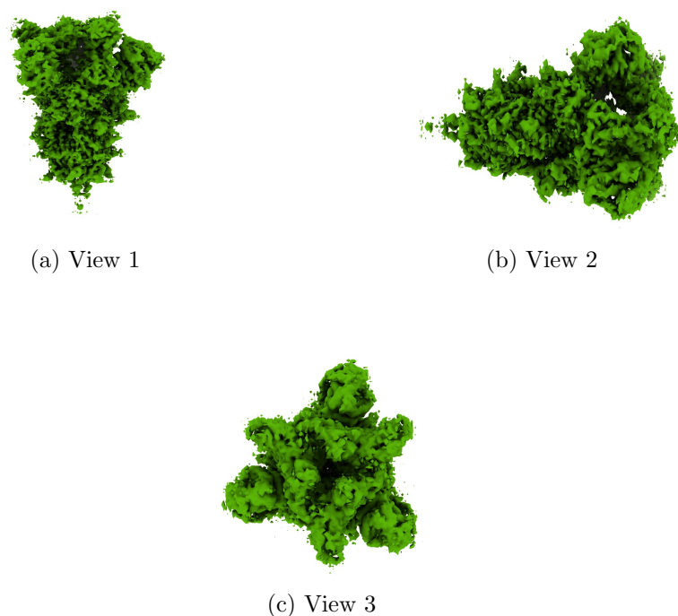
Figure 4: Isosurface at threshold=0.271000. Views generated by ChimeraX at a the following X, Y, Z angles: View 1 (0, -90, -90), View 2 (-90, 0, -90), View 3 (0, 0, 0).
