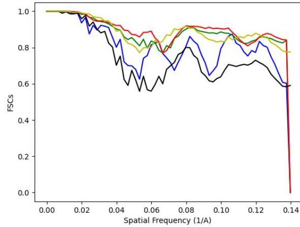
Figure 28: FSC in X, Y, Z, the global FSC, and the Average Cosine Phase.
