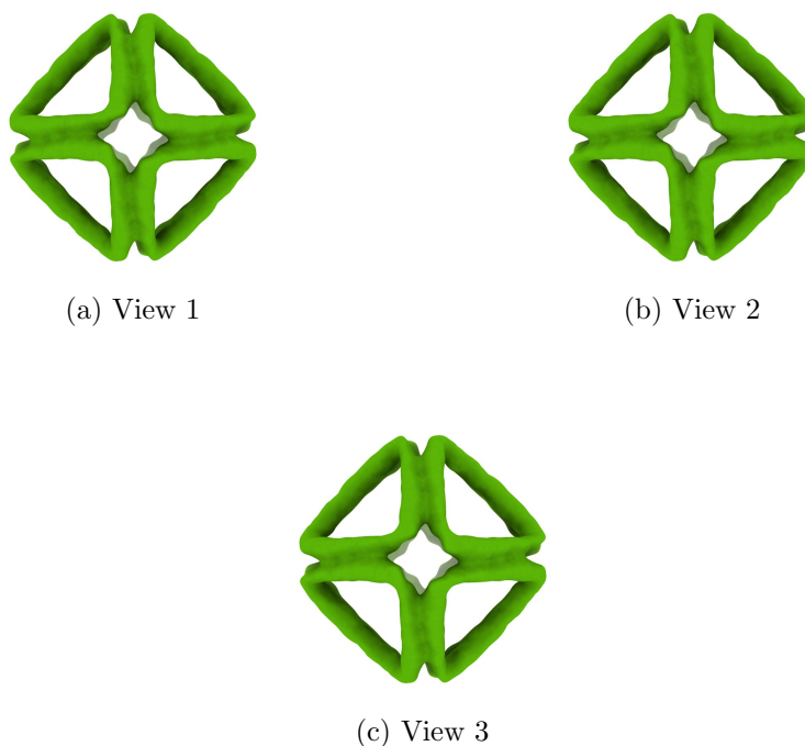
Figure 4: Isosurface at threshold=0.490000. Views generated by ChimeraX at a the following X, Y, Z angles: View 1 (0, -90, -90), View 2 (-90, 0, -90), View 3 (0, 0, 0).
