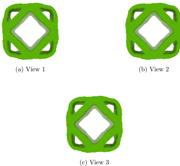
Figure 4: Isosurface at threshold=0.565000. Views generated by ChimeraX at a the following X, Y, Z angles: View 1 (0, -90, -90), View 2 (-90, 0, -90), View 3 (0, 0, 0).
