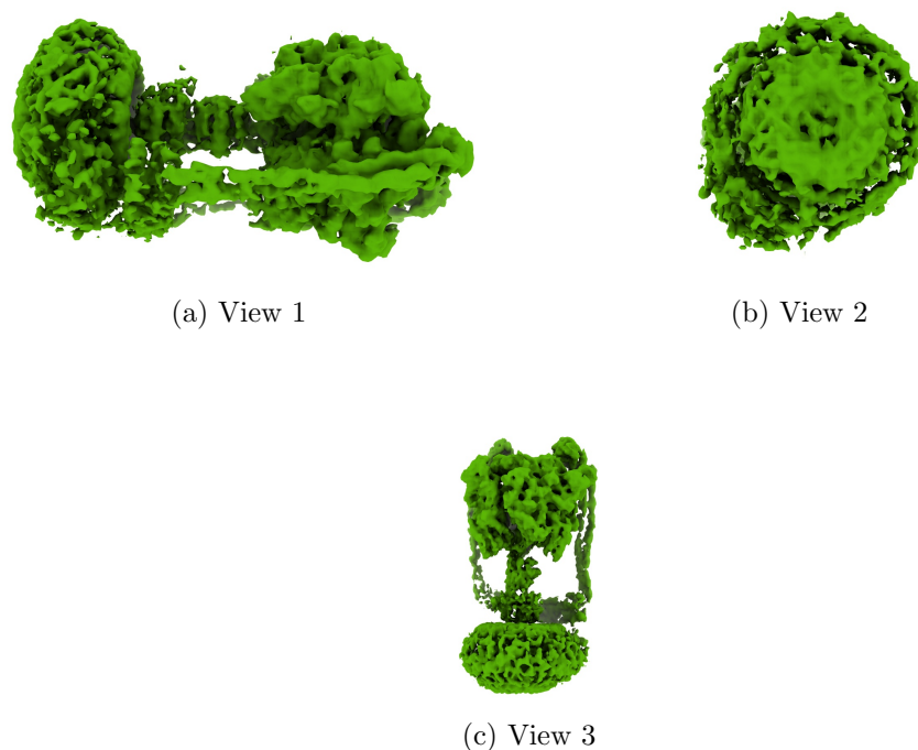
Figure 4: Isosurface at threshold=0.005000. Views generated by ChimeraX at a the following X, Y, Z angles: View 1 (0, -90, -90), View 2 (-90, 0, -90), View 3 (0, 0, 0).
