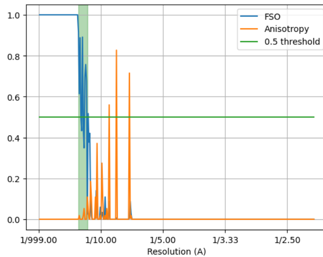
Figure 20: FSO and anisotropy.
