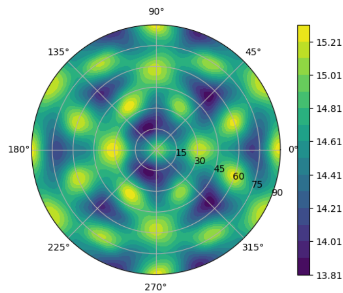
Figure 21: Directional resolution in the projection sphere.
