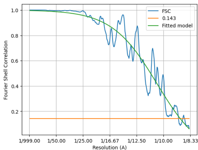
Figure 15: Fourier Shell correlation between the two halves.
