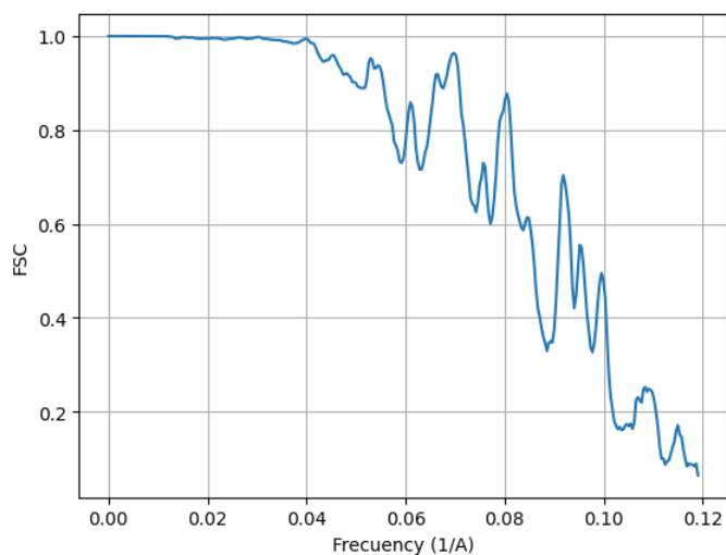
Figure 18: FSC and resolution estimated by a permutation test.
