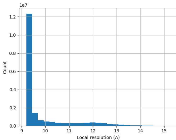
Figure 21: Histogram of the local resolution according to Resmap.
