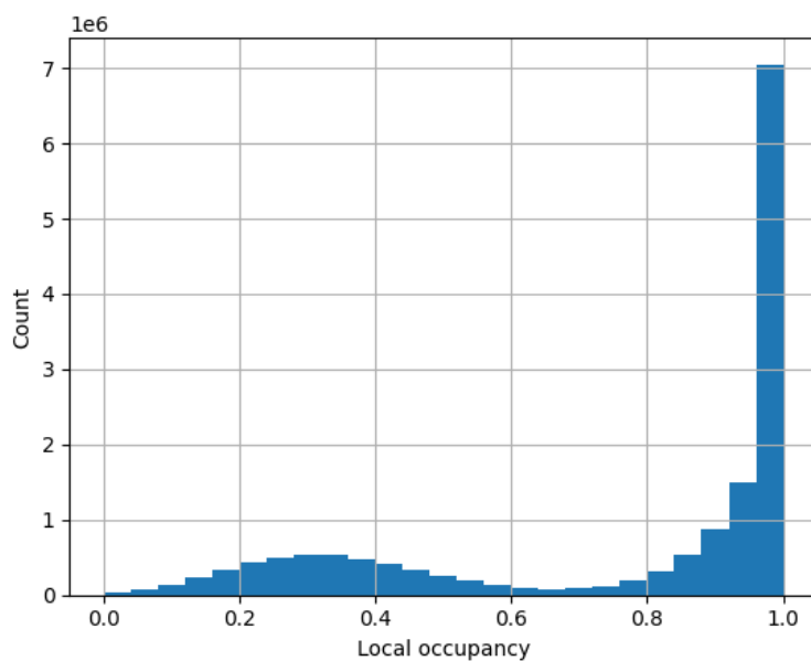
Figure 10: Histogram of the local occupancy according to LocOccupancy.
