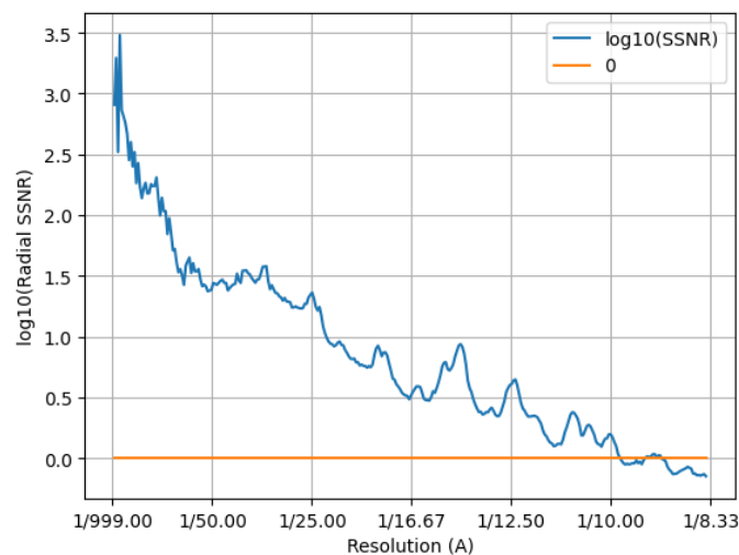
Figure 17: Spectral Signal-to-Noise Ratio estimated from the two halves.
