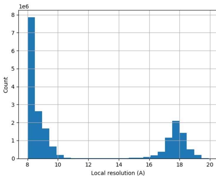
Figure 19: Histogram of the local resolution according to blocres.
