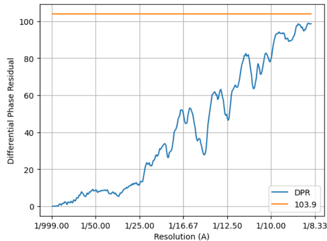
Figure 16: Differential Phase Residual between the two halves.
