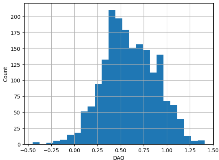
Figure 49: Histogram of the per-residue DAQ values.
