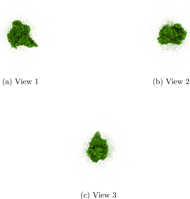
Figure 4: Isosurface at threshold=0.136000. Views generated by ChimeraX at a the following X, Y, Z angles: View 1 (0, -90, -90), View 2 (-90, 0, -90), View 3 (0, 0, 0).
