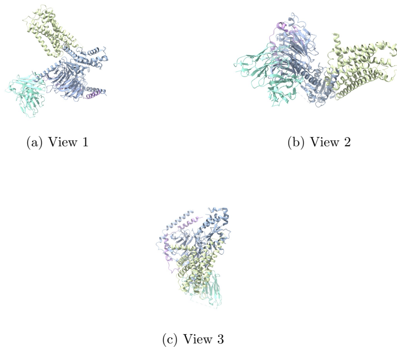
Figure 34: Input atomic model Views generated by ChimeraX at a the following X, Y, Z angles: View 1 (0, -90, -90), View 2 (-90, 0, -90), View 3 (0, 0, 0).
