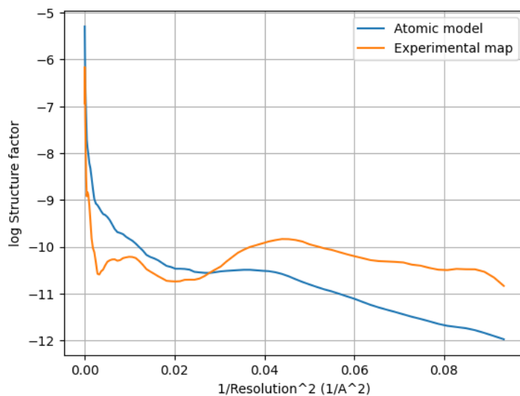
Figure 44: Guinier plot of the atom model and experimental map. The X-axis is the square of the inverse of the resolution in Å.
