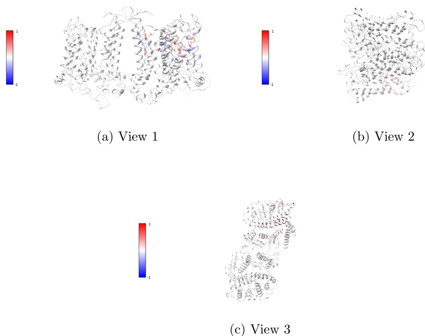
Figure 46: Atomic model colored by MapQ Views generated by ChimeraX at a the following X, Y, Z angles: View 1 (0, -90, -90), View 2 (-90, 0, -90), View 3 (0, 0, 0).
