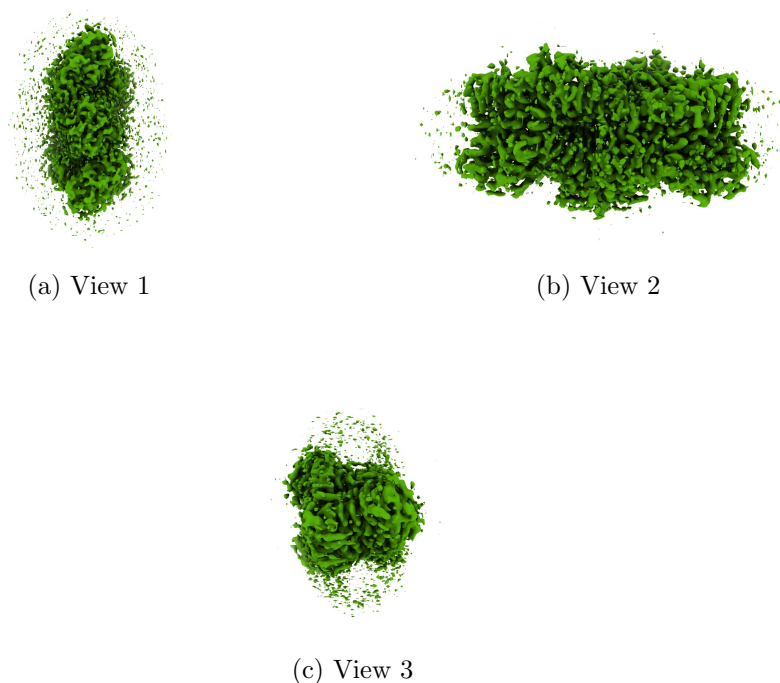
Figure 4: Isosurface at threshold=0.600000. Views generated by ChimeraX at a the following X, Y, Z angles: View 1 (0, -90, -90), View 2 (-90, 0, -90), View 3 (0, 0, 0).
