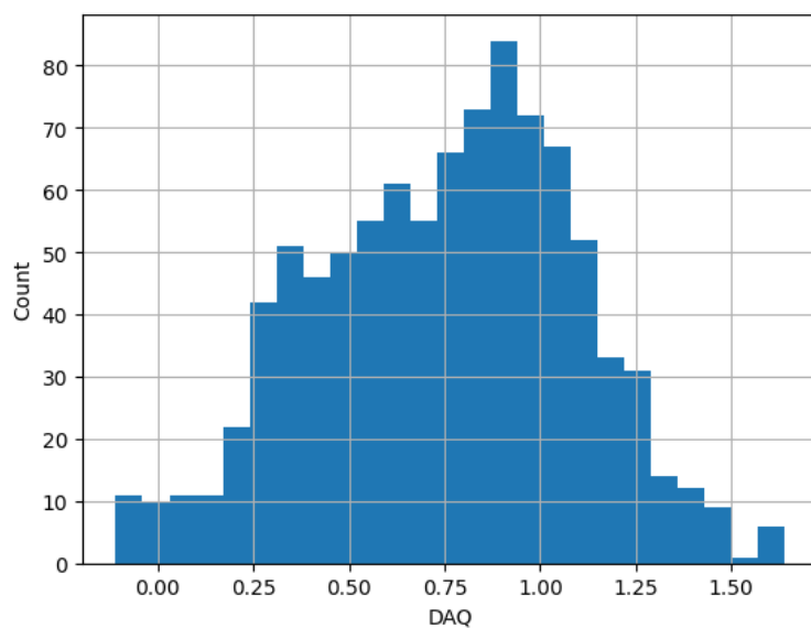
Figure 46: Histogram of the per-residue DAQ values.
