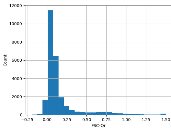
Figure 39: Histogram of the FSC-Qr limited to -1.5 and 1.5.
