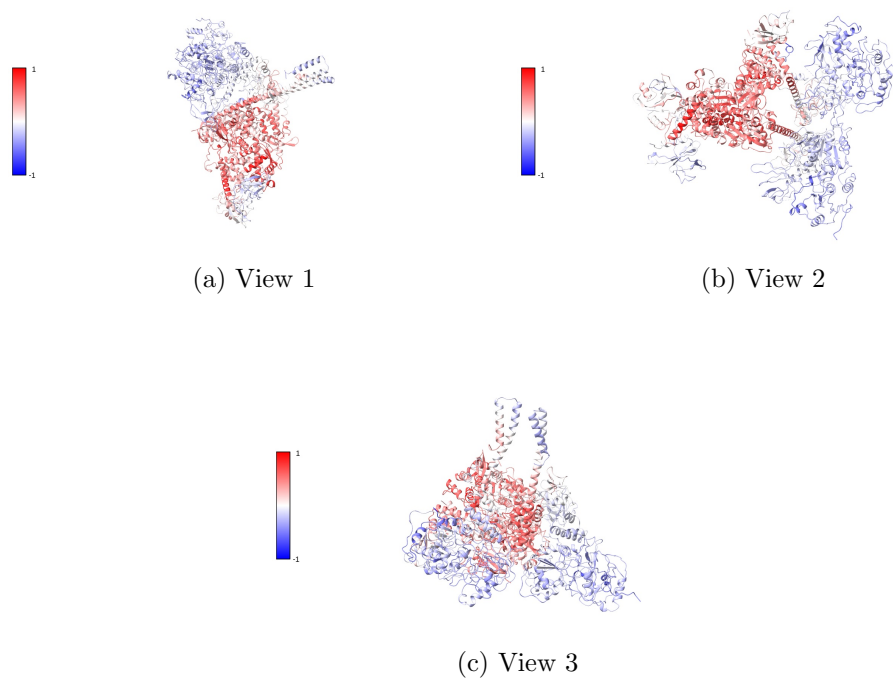
Figure 48: Atomic model colored by DAQ Views generated by ChimeraX at the following X, Y, Z angles: View 1 (0, -90, -90), View 2 (-90, 0, -90), View 3 (0, 0, 0).
