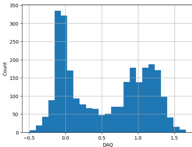
Figure 47: Histogram of the per-residue DAQ values.
