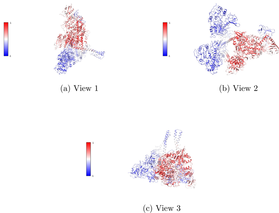
Figure 48: Atomic model colored by DAQ Views generated by ChimeraX at the following X, Y, Z angles: View 1 (0, -90, -90), View 2 (-90, 0, -90), View 3 (0, 0, 0).
