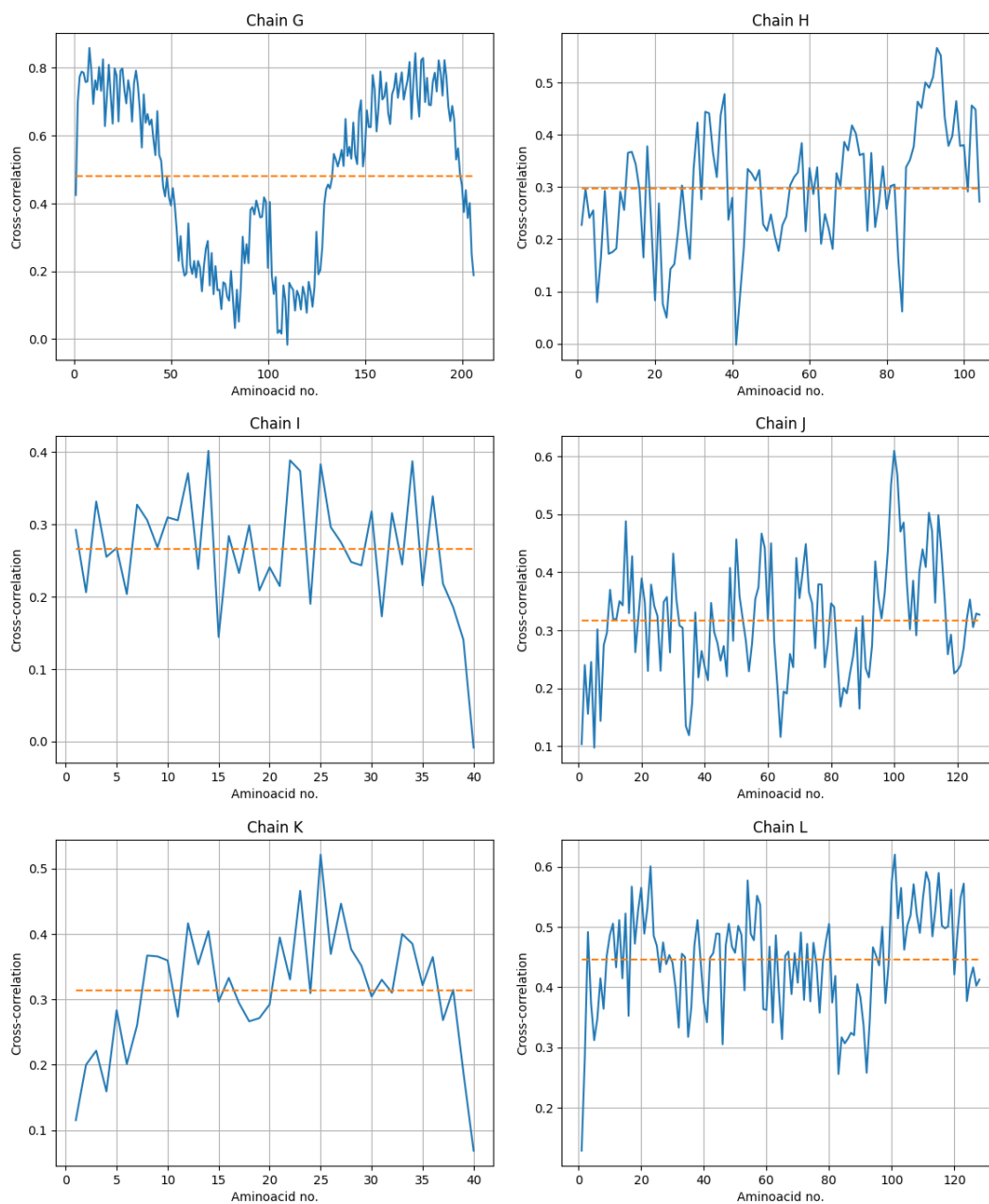
Fig. 37 shows the histogram of all cross-correlations evaluated at the residues. The percentage of residues whose correlation is below 0.5 is 15.4 %.
