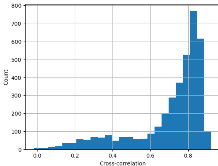
Figure 37: Histogram of the cross-correlation between the map and model evaluated for all residues.
