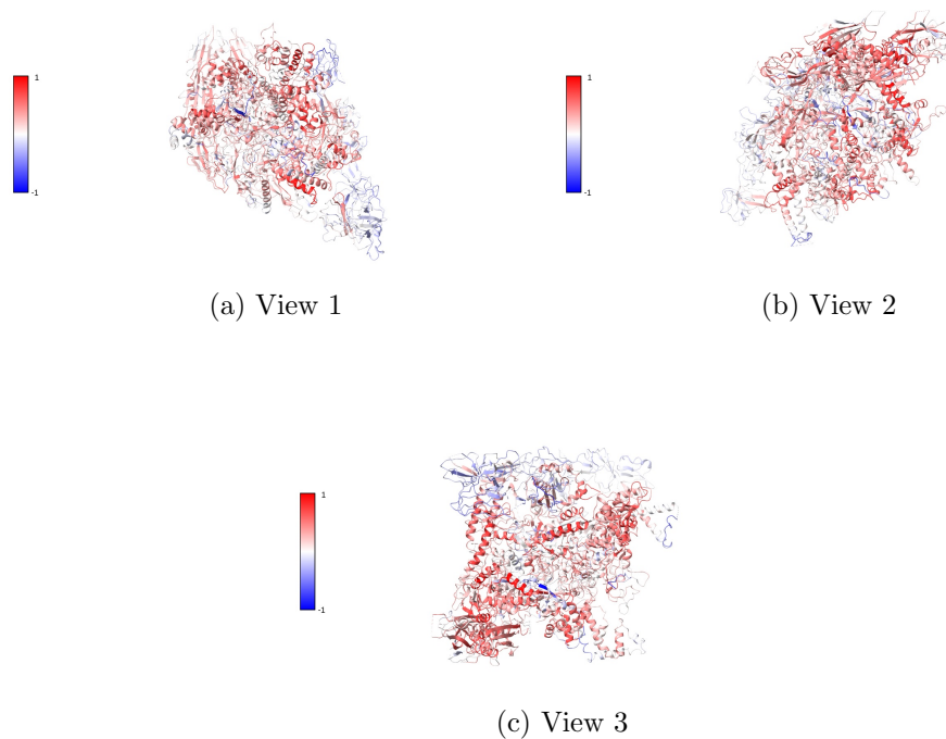
Figure 47: Atomic model colored by DAQ Views generated by ChimeraX at the following X, Y, Z angles: View 1 (0, -90, -90), View 2 (-90, 0, -90), View 3 (0, 0, 0).
