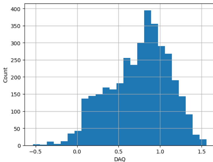
Figure 46: Histogram of the per-residue DAQ values.
