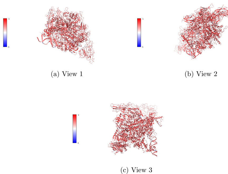
Figure 43: Atomic model colored by MapQ Views generated by ChimeraX at a the following X, Y, Z angles: View 1 (0, -90, -90), View 2 (-90, 0, -90), View 3 (0, 0, 0).
