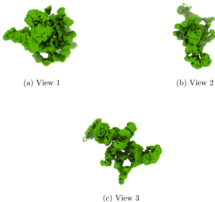
Figure 4: Isosurface at threshold=0.008050. Views generated by ChimeraX at a the following X, Y, Z angles: View 1 (0, -90, -90), View 2 (-90, 0, -90), View 3 (0, 0, 0).
