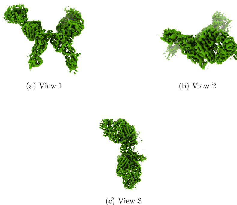
Figure 4: Isosurface at threshold=0.400600. Views generated by ChimeraX at a the following X, Y, Z angles: View 1 (0, -90, -90), View 2 (-90, 0, -90), View 3 (0, 0, 0).
