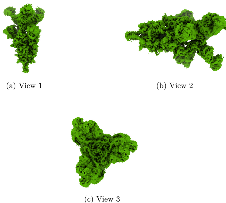
Figure 4: Isosurface at threshold=0.220600. Views generated by ChimeraX at a the following X, Y, Z angles: View 1 (0, -90, -90), View 2 (-90, 0, -90), View 3 (0, 0, 0).
