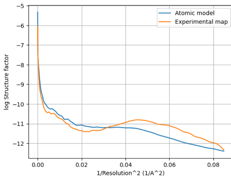
Figure 42: Guinier plot of the atom model and experimental map. The X-axis is the square of the inverse of the resolution in Å.
