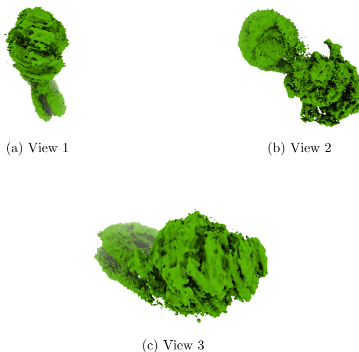
Figure 4: Isosurface at threshold=0.016000. Views generated by ChimeraX at a the following X, Y, Z angles: View 1 (0, -90, -90), View 2 (-90, 0, -90), View 3 (0, 0, 0).
