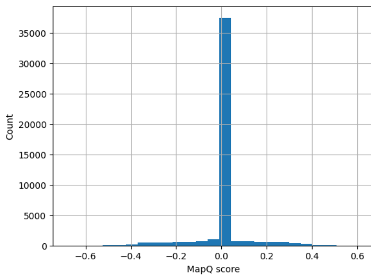
Figure 45: Histogram of the per-atom Q-score.
