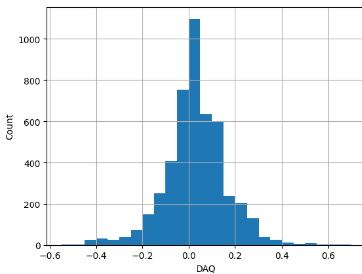
Figure 49: Histogram of the per-residue DAQ values.
