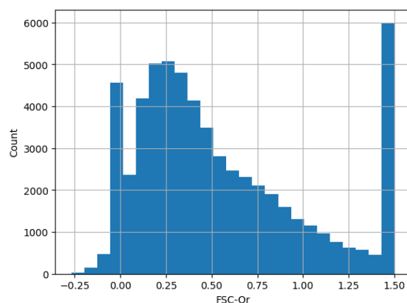
Figure 42: Histogram of the FSC-Qr limited to -1.5 and 1.5.
