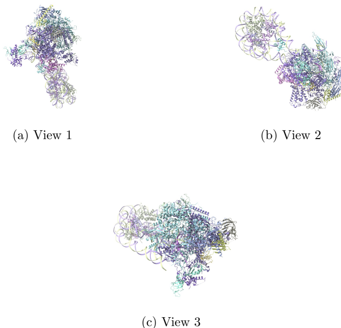
Figure 39: Input atomic model Views generated by ChimeraX at a the following X, Y, Z angles: View 1 (0, -90, -90), View 2 (-90, 0, -90), View 3 (0, 0, 0).
