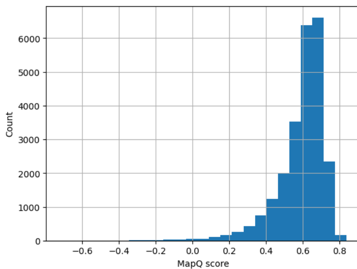
Figure 43: Histogram of the per-atom Q-score.
