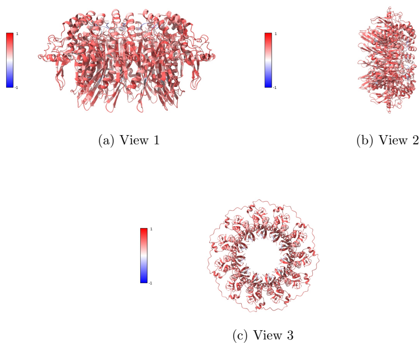
Figure 43: Atomic model colored by MapQ Views generated by ChimeraX at a the following X, Y, Z angles: View 1 (0, -90, -90), View 2 (-90, 0, -90), View 3 (0, 0, 0).
