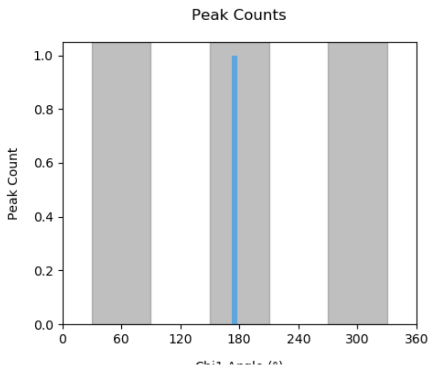
Figure 44: Histogram for rotameric (blue) and non-rotameric (red) residues at the optimal threshold as a function of the angle Chi1.
