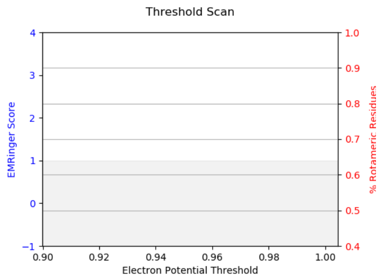
Figure 43: EMRinger score and fraction of rotameric residues as a function of the map threshold.
