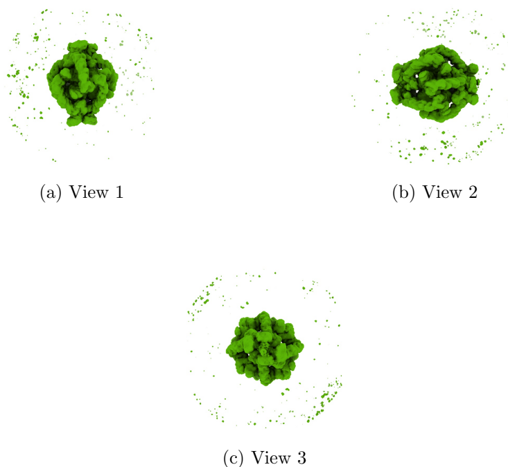
Figure 4: Isosurface at threshold=0.001000. Views generated by ChimeraX at a the following X, Y, Z angles: View 1 (0, -90, -90), View 2 (-90, 0, -90), View 3 (0, 0, 0).
