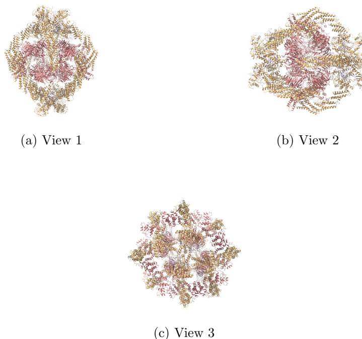
Figure 37: Input atomic model Views generated by ChimeraX at a the following X, Y, Z angles: View 1 (0, -90, -90), View 2 (-90, 0, -90), View 3 (0, 0, 0).
