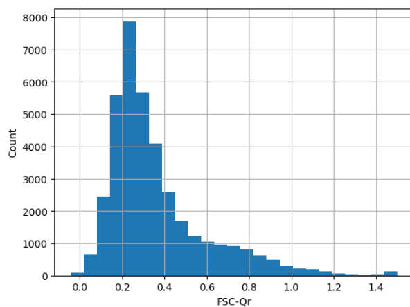
Figure 40: Histogram of the FSC-Qr limited to -1.5 and 1.5.
