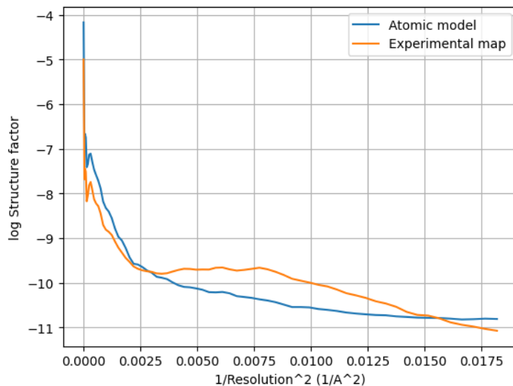
Figure 42: Guinier plot of the atom model and experimental map. The X-axis is the square of the inverse of the resolution in Å.
