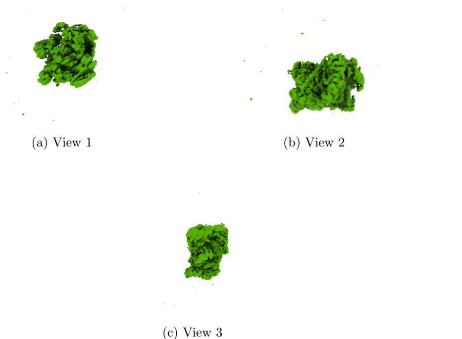
Figure 4: Isosurface at threshold=0.001000. Views generated by ChimeraX at a the following X, Y, Z angles: View 1 (0, -90, -90), View 2 (-90, 0, -90), View 3 (0, 0, 0).
