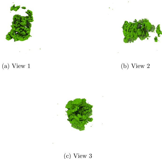
Figure 4: Isosurface at threshold=0.001000. Views generated by ChimeraX at a the following X, Y, Z angles: View 1 (0, -90, -90), View 2 (-90, 0, -90), View 3 (0, 0, 0).
