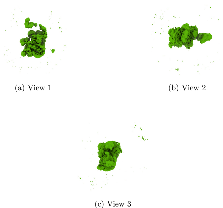
Figure 4: Isosurface at threshold=0.001000. Views generated by ChimeraX at a the following X, Y, Z angles: View 1 (0, -90, -90), View 2 (-90, 0, -90), View 3 (0, 0, 0).
