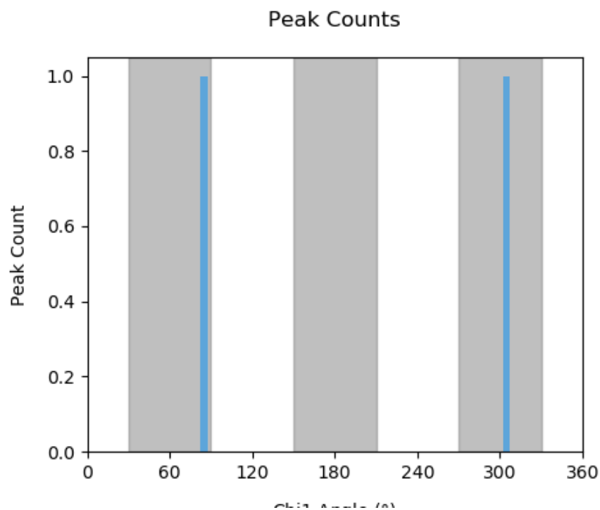
Figure 46: Histogram for rotameric (blue) and non-rotameric (red) residues at the optimal threshold as a function of the angle Chi1.
