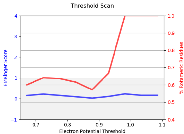
Figure 45: EMRinger score and fraction of rotameric residues as a function of the map threshold.
