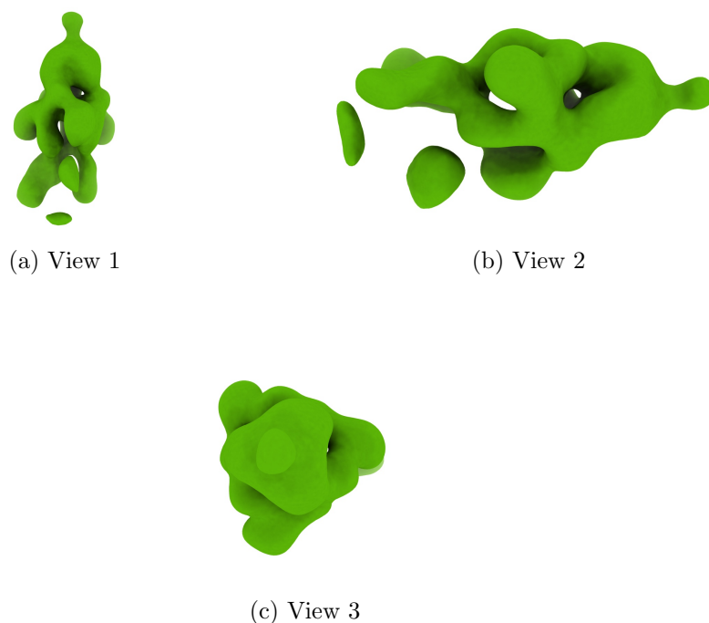
Figure 4: Isosurface at threshold=0.030700. Views generated by ChimeraX at a the following X, Y, Z angles: View 1 (0, -90, -90), View 2 (-90, 0, -90), View 3 (0, 0, 0).
