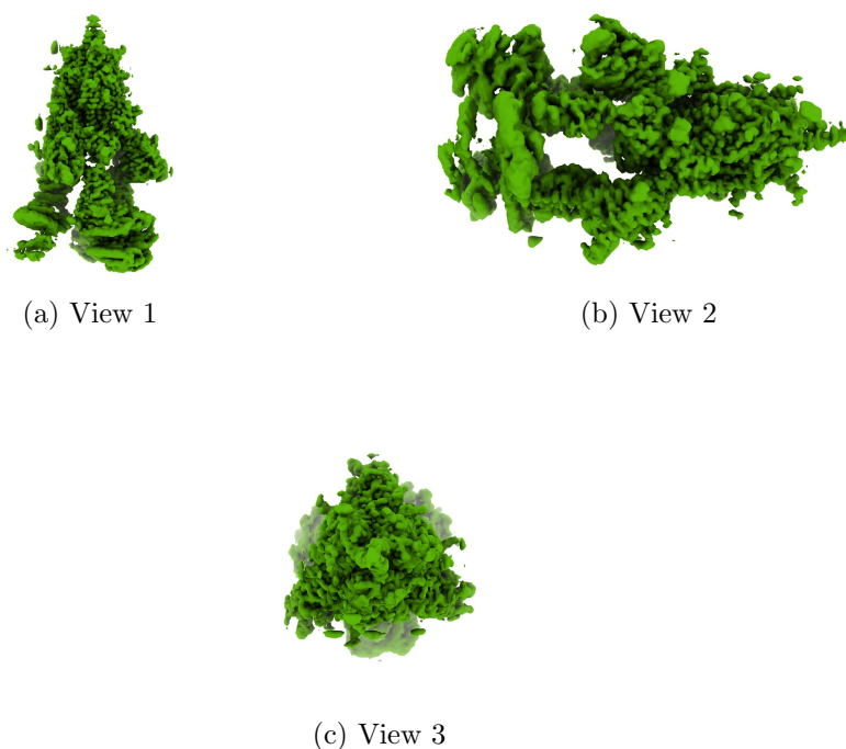
Figure 4: Isosurface at threshold=0.018500. Views generated by ChimeraX at a the following X, Y, Z angles: View 1 (0, -90, -90), View 2 (-90, 0, -90), View 3 (0, 0, 0).
