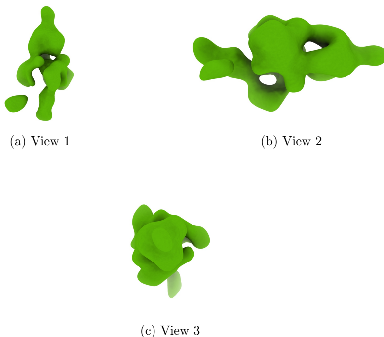
Figure 4: Isosurface at threshold=0.032300. Views generated by ChimeraX at a the following X, Y, Z angles: View 1 (0, -90, -90), View 2 (-90, 0, -90), View 3 (0, 0, 0).
