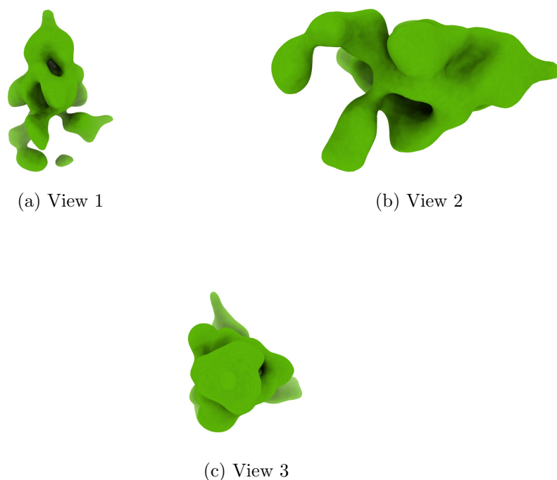
Figure 4: Isosurface at threshold=0.021500. Views generated by ChimeraX at the following X, Y, Z angles: View 1 (0, -90, -90), View 2 (-90, 0, -90), View 3 (0, 0, 0).
