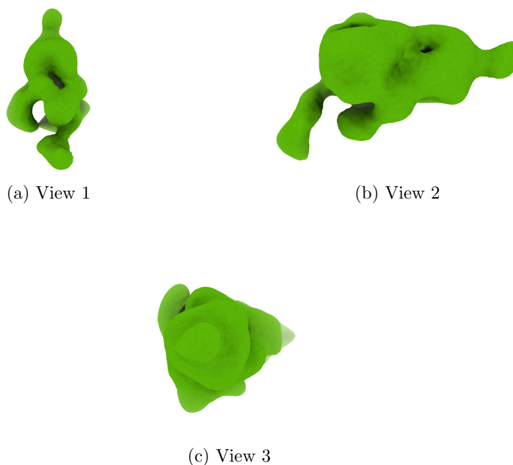
Figure 4: Isosurface at threshold=0.029600. Views generated by ChimeraX at a the following X, Y, Z angles: View 1 (0, -90, -90), View 2 (-90, 0, -90), View 3 (0, 0, 0).
