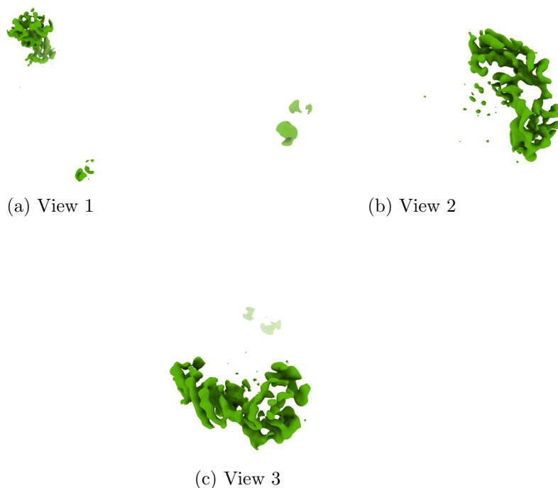
Figure 4: Isosurface at threshold=0.140000. Views generated by ChimeraX at a the following X, Y, Z angles: View 1 (0, -90, -90), View 2 (-90, 0, -90), View 3 (0, 0, 0).
