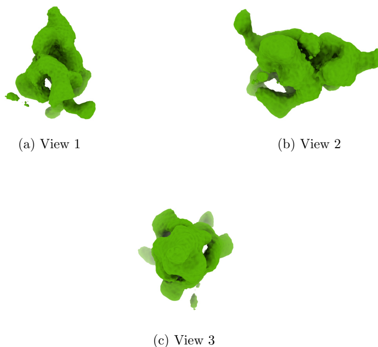
Figure 4: Isosurface at threshold=0.020200. Views generated by ChimeraX at a the following X, Y, Z angles: View 1 (0, -90, -90), View 2 (-90, 0, -90), View 3 (0, 0, 0).
