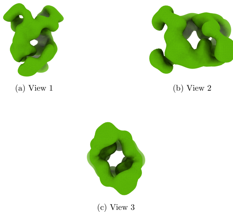
Figure 4: Isosurface at threshold=1.120000. Views generated by ChimeraX at a the following X, Y, Z angles: View 1 (0, -90, -90), View 2 (-90, 0, -90), View 3 (0, 0, 0).
