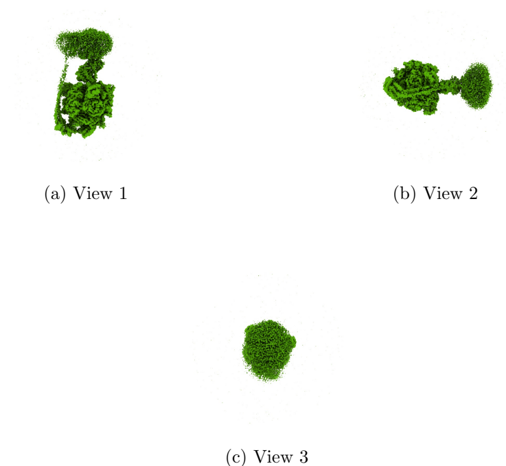
Figure 4: Isosurface at threshold=0.004700. Views generated by ChimeraX at a the following X, Y, Z angles: View 1 (0, -90, -90), View 2 (-90, 0, -90), View 3 (0, 0, 0).
