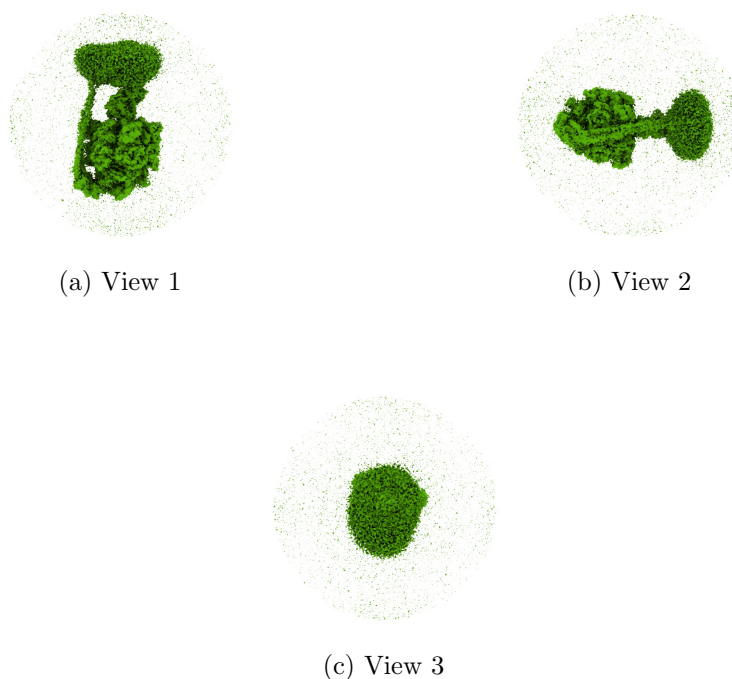
Figure 4: Isosurface at threshold=0.003910. Views generated by ChimeraX at a the following X, Y, Z angles: View 1 (0, -90, -90), View 2 (-90, 0, -90), View 3 (0, 0, 0).
