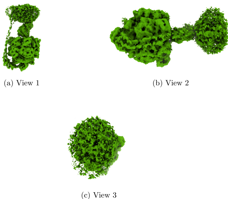
Figure 4: Isosurface at threshold=0.004700. Views generated by ChimeraX at a the following X, Y, Z angles: View 1 (0, -90, -90), View 2 (-90, 0, -90), View 3 (0, 0, 0).
