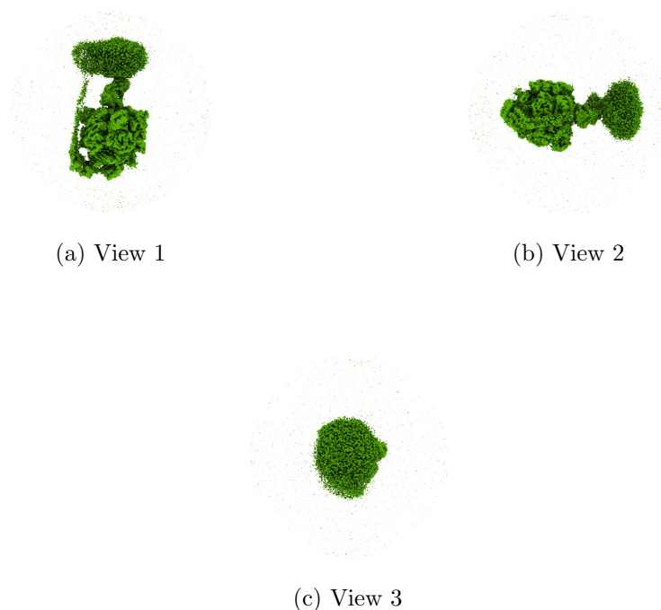
Figure 4: Isosurface at threshold=0.004100. Views generated by ChimeraX at a the following X, Y, Z angles: View 1 (0, -90, -90), View 2 (-90, 0, -90), View 3 (0, 0, 0).
