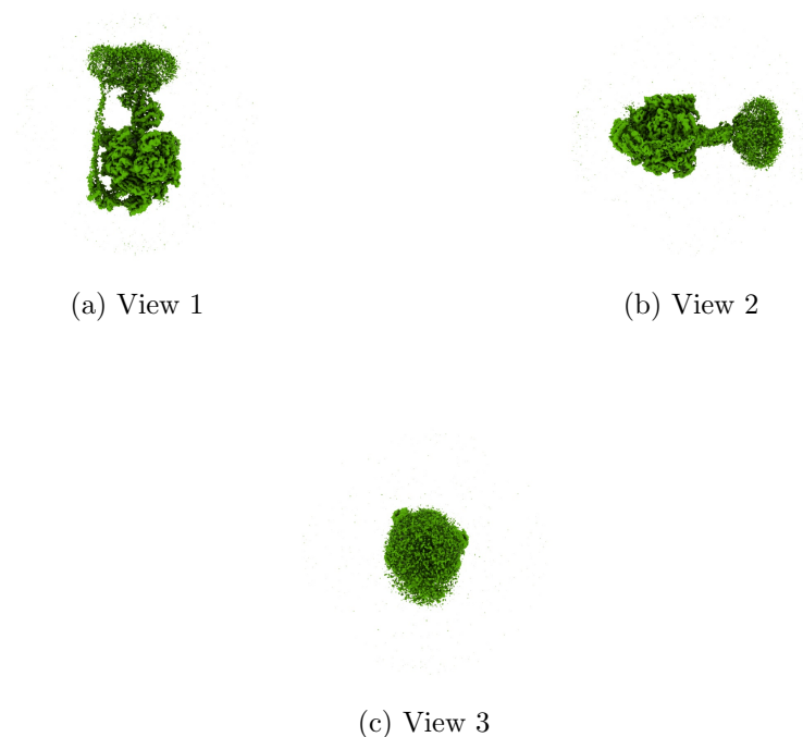
Figure 4: Isosurface at threshold=0.005180. Views generated by ChimeraX at a the following X, Y, Z angles: View 1 (0, -90, -90), View 2 (-90, 0, -90), View 3 (0, 0, 0).
