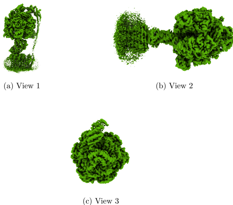
Figure 4: Isosurface at threshold=0.005720. Views generated by ChimeraX at a the following X, Y, Z angles: View 1 (0, -90, -90), View 2 (-90, 0, -90), View 3 (0, 0, 0).
